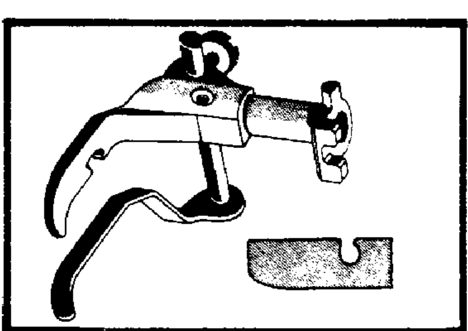
EDGE FOOT WITH ADJUSTABLE GUIDE For straight stitch sewing on edge of material; piping or quilting. No. 530615 For all models.
