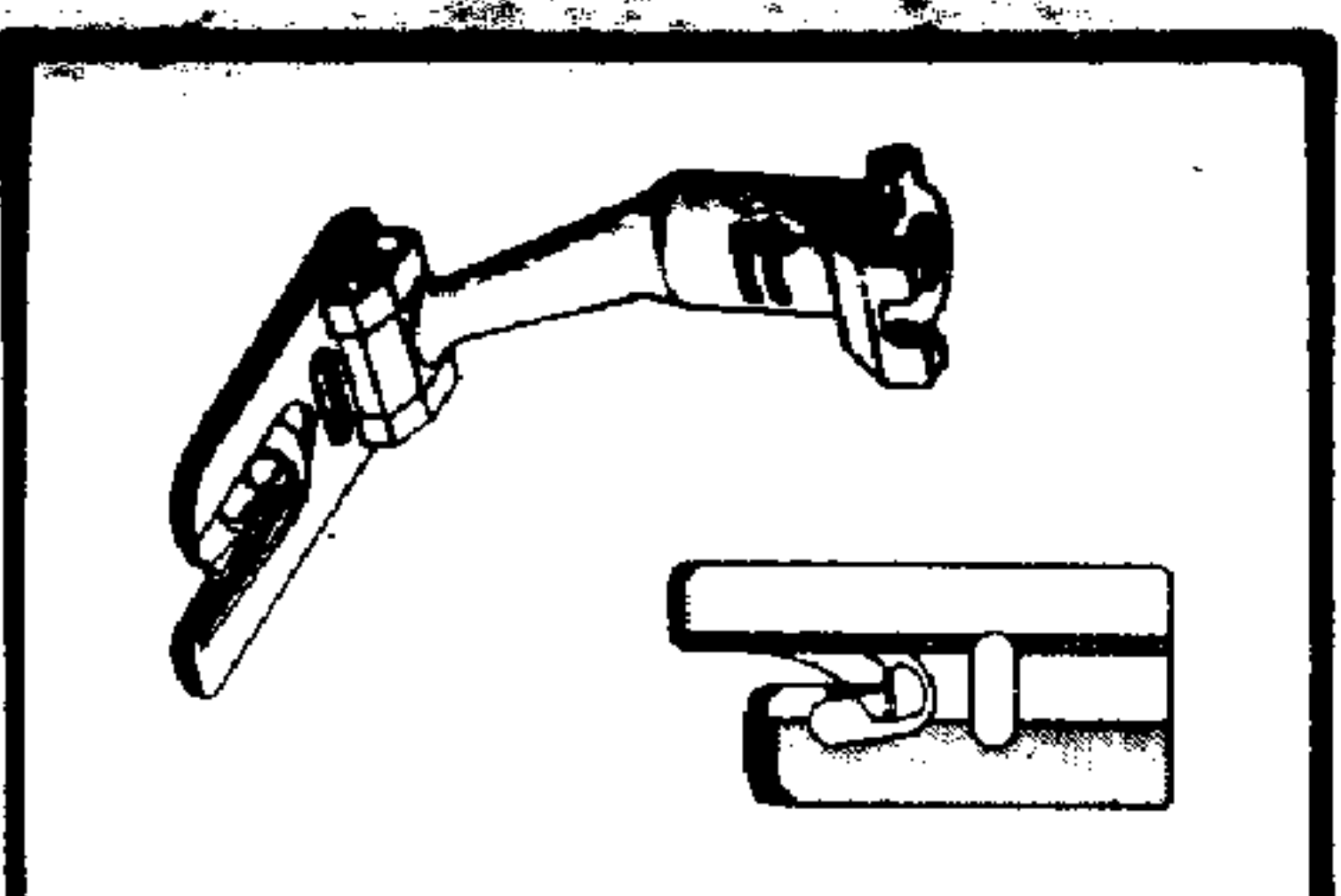
ROLL AND SHELL HEMMER FOOT For making a shell edge or hemming edges with decorative zig zag stitches on either side of hem. No. 530611 For Swing Needle and Automatic Models.
